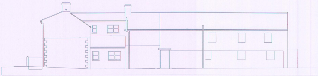
EAST ELEVATION
